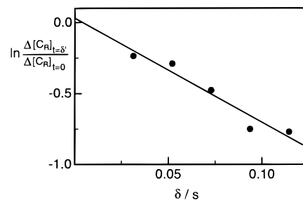
Figure 2. Semilogarithmic plot of \Delta[C_r]_{t=\delta}/\Delta[C_r]_{t=0} versus the delay time \delta which is given by \delta = \delta' + \Delta t/2 to account for the width of the measuring interval.
