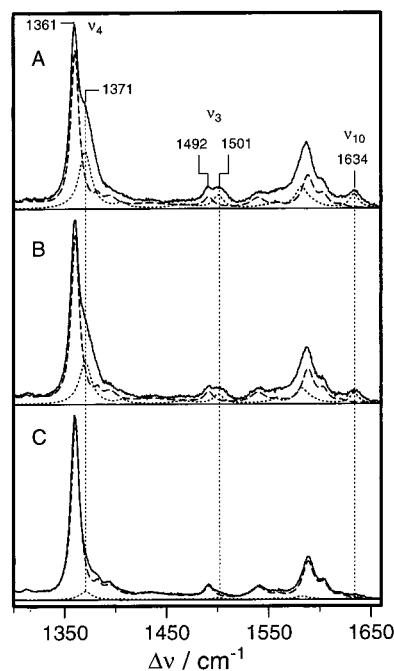
Figure 1. Time-resolved SERR spectra of Cyt- c 552 measured at delay times of 21 (A) and 62 ms (B) following a potential jump from 0.0 to -0.1 V, compared with a stationary SERR spectrum measured at -0.1 V (C). Excitation wavelength: 413 nm ( 50 mW at the sample). Spectral resolution: 2.5\text{ cm}^{-1} with 0.5\text{ cm}^{-1} increments per data point. Accumulation time: 20 s for C and 3 s for A and B. The component spectra of the oxidized and reduced state B1 are denoted by the dotted and dashed lines, respectively. For simplicity, the component spectra of state B2 which contribute by less than 10\% to the measured spectra are not displayed.
